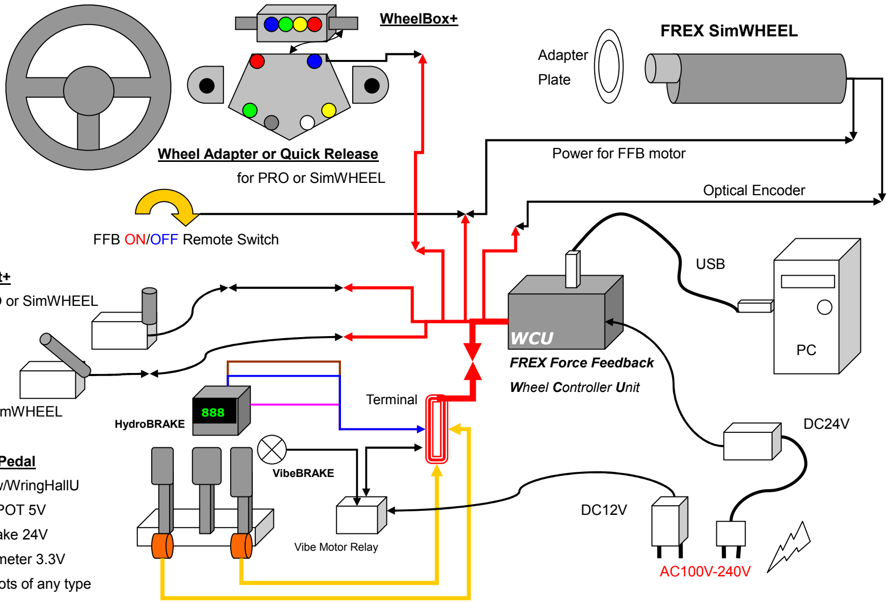
FREX SimWHEEL Force Feedback Wheel Wiring Diagram v1.0 2008.02.20
